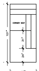
LOUNGER GRAND W: 46" D: 101" H: 30" SEAT D: 28"
