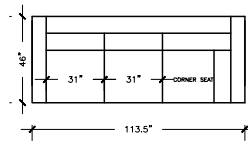
SOFA PLUS D W: 113.5" D: 46" H: 30" ARM H: 23" SEAT D: 28"
