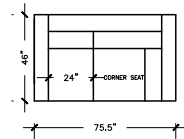
LOVE SEAT D W: 75.5" D: 46" H: 30" ARM H: 23" SEAT D: 28"
