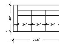
SOFA B W: 79.5" D: 46" H: 30" ARM H: 23" SEAT D: 28"
