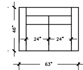
LOVE SEAT W: 63" D: 46" H: 30" ARM H: 23" SEAT D: 28"
