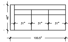
SOFA PLUS B W: 100.5" D: 46" H: 30" ARM H: 23" SEAT D: 28"
